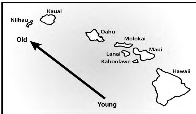
Figure 12. The Hawaiian Islands formed over a hotspot.
