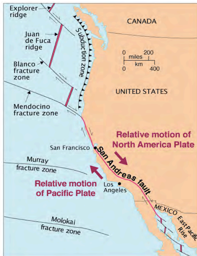
Figure 10. The San Andreas Fault
