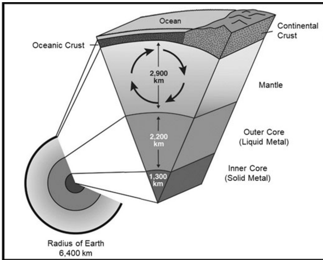
Figure 2. Simple diagram of Earth's interior
