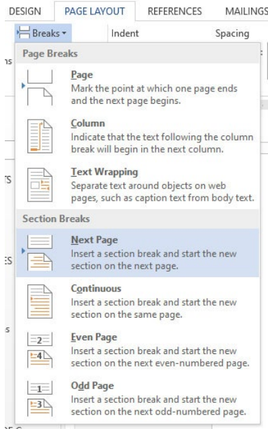
Figure 22: Section break
