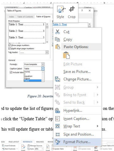
Figure 27: Format picture
