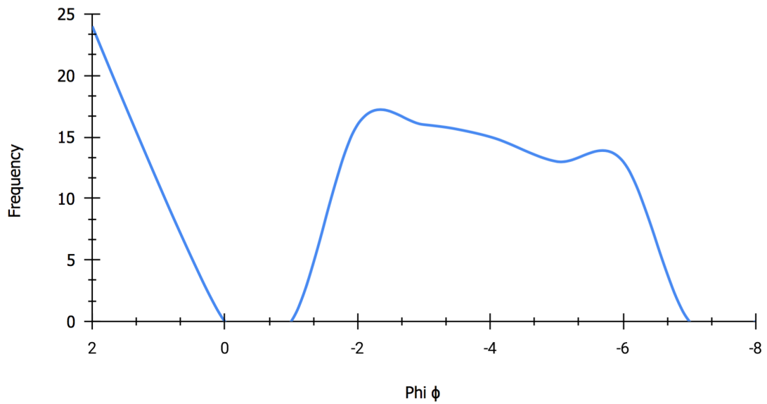
Appendix B. 36. West - Phi vs. Frequency individual graphs (CC14) Unit L.
