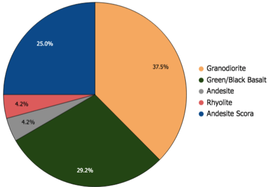
Appendix B. 65. Tadpole Tank- Clast Composition individual pie charts with key (CC20) Unit BT.
