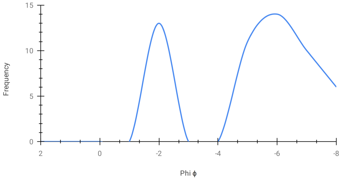
Appendix B. 43. West - Phi vs. Frequency individual graphs (CC20) Unit R.
