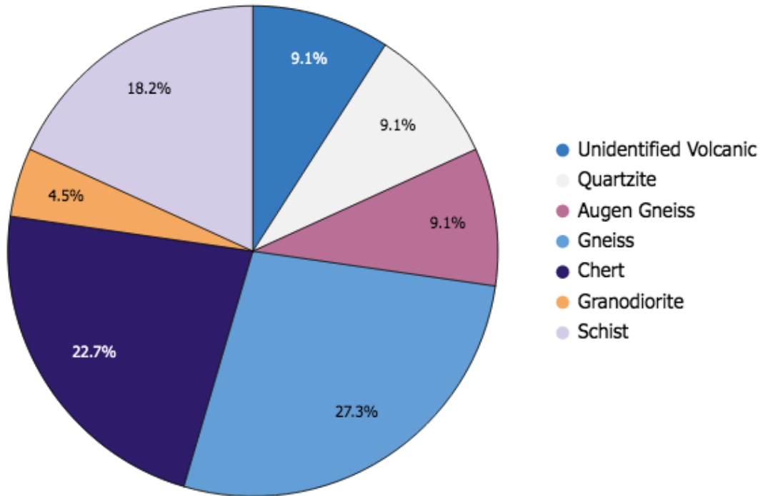
Appendix B. 47. West - Clast Composition individual pie charts with key (CC4) Unit R VRSS.
