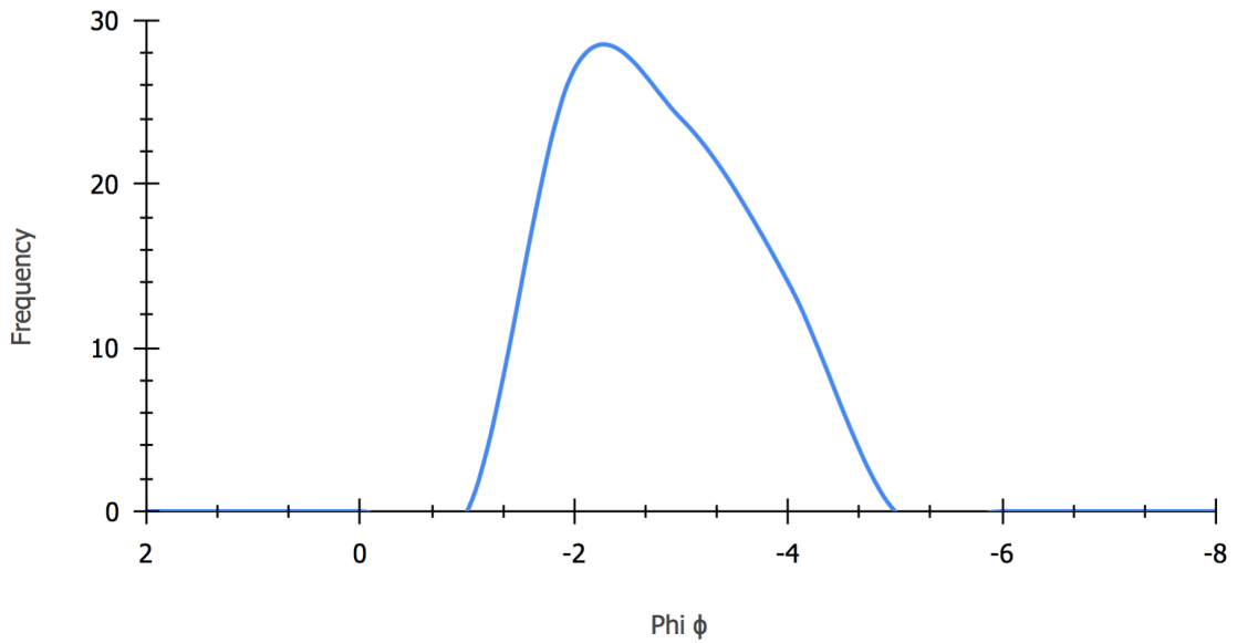
Appendix B. 38. West - Phi vs. Frequency individual graphs (CC16) Unit R.
