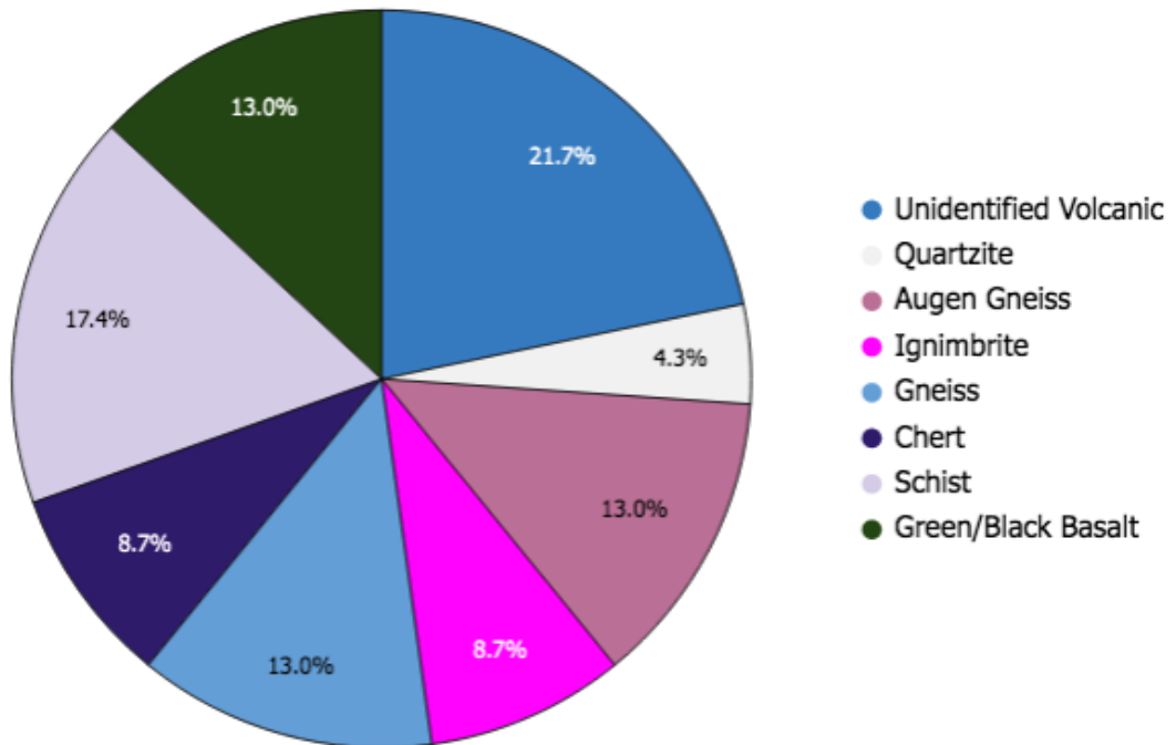
Appendix B. 58. East - Clast Composition individual pie charts with key (CC14) Unit L.
