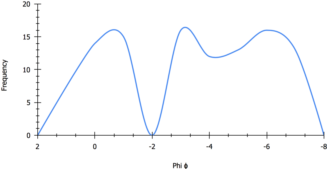
Appendix B. 31. West - Phi vs. Frequency individual graphs (CC10) Unit R.
