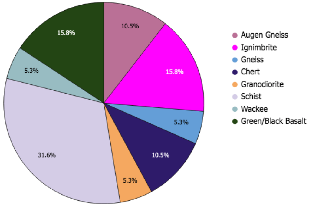
Appendix B. 57. East - Clast Composition individual pie charts with key (CC13) Unit R DRSS.
