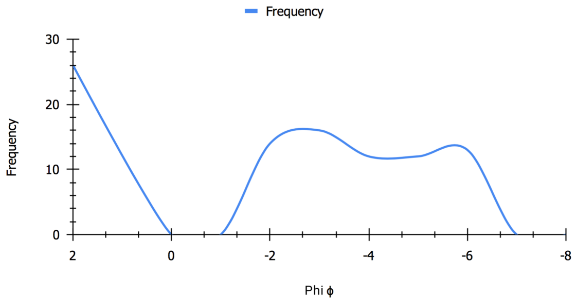
Appendix B. 26. West - Phi vs. Frequency individual graphs (CC5) Unit L.
