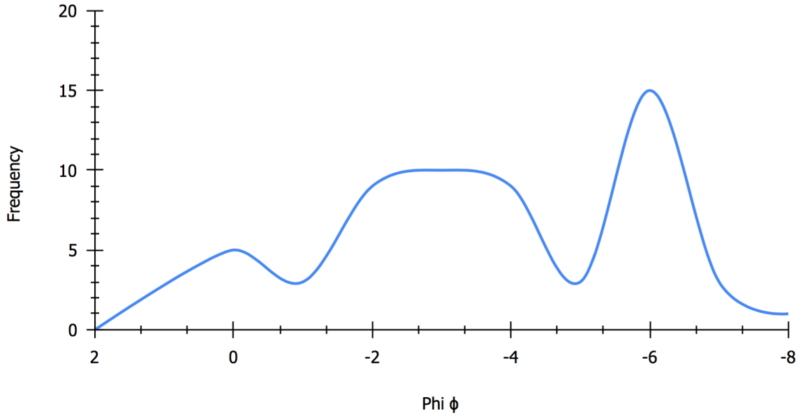
Appendix B. 23. West - Phi vs. Frequency individual graphs (CC2) Unit R.
