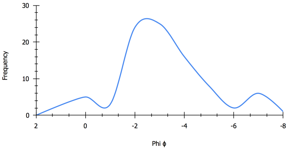
Appendix B. 42. West - Phi vs. Frequency individual graphs (CC1) Unit R.
