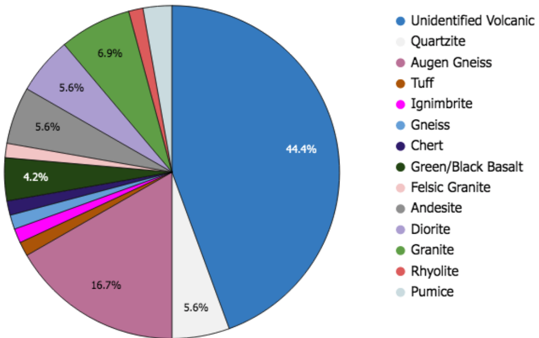
Appendix B. 64. Tadpole Tank- Clast Composition individual pie charts with key (CC1) Unit R ORSS.
