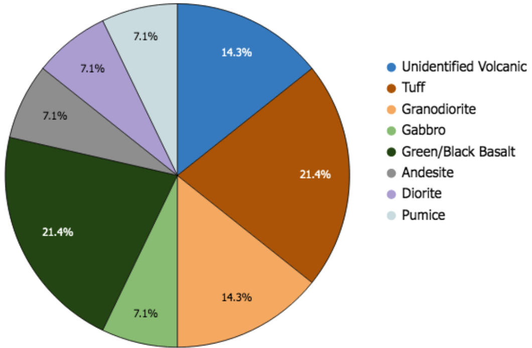
Appendix B. 49. West - Clast Composition individual pie charts with key (CC6) Unit R DRSS.
