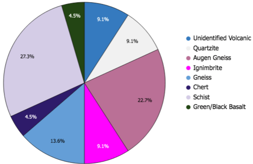
Appendix B. 63. East - Clast Composition individual pie charts with key (CC19) Unit L.
