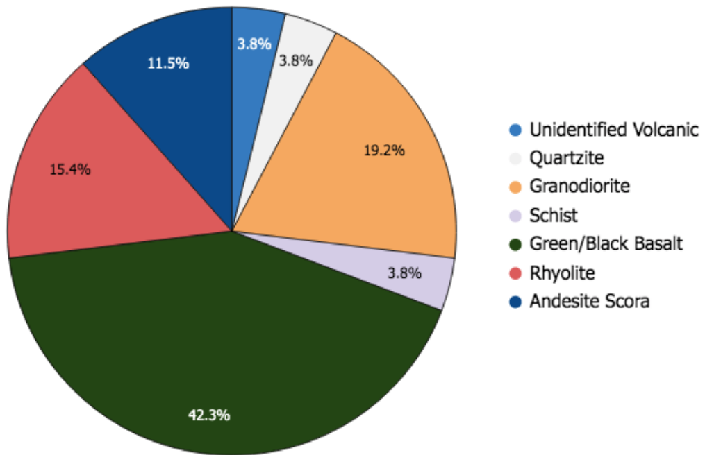
Appendix B. 66. Tadpole Tank- Clast Composition individual pie charts with key (CC21) Unit BT.
