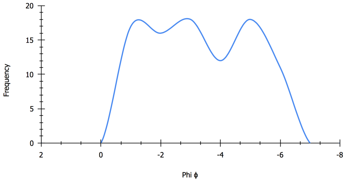
Appendix B. 35. West - Phi vs. Frequency individual graphs (CC13) Unit R.
