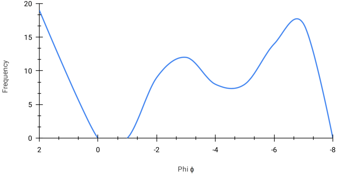
Appendix B. 30. West - Phi vs. Frequency individual graphs (CC9) Unit L.
