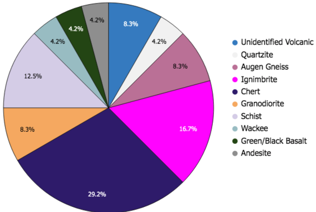
Appendix B. 56. East - Clast Composition individual pie charts with key (CC12) Unit R DRSS.
