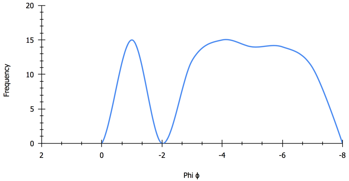
Appendix B. 25. West - Phi vs. Frequency individual graphs (CC4) Unit R.
