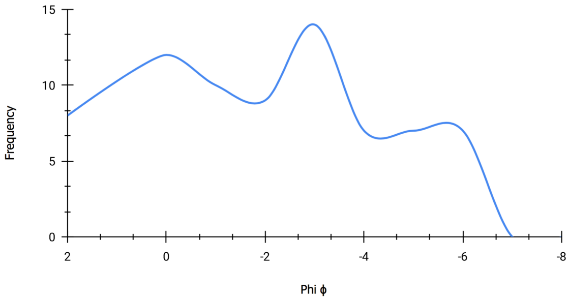
Appendix B. 28. West - Phi vs. Frequency individual graphs (CC7) Unit R.
