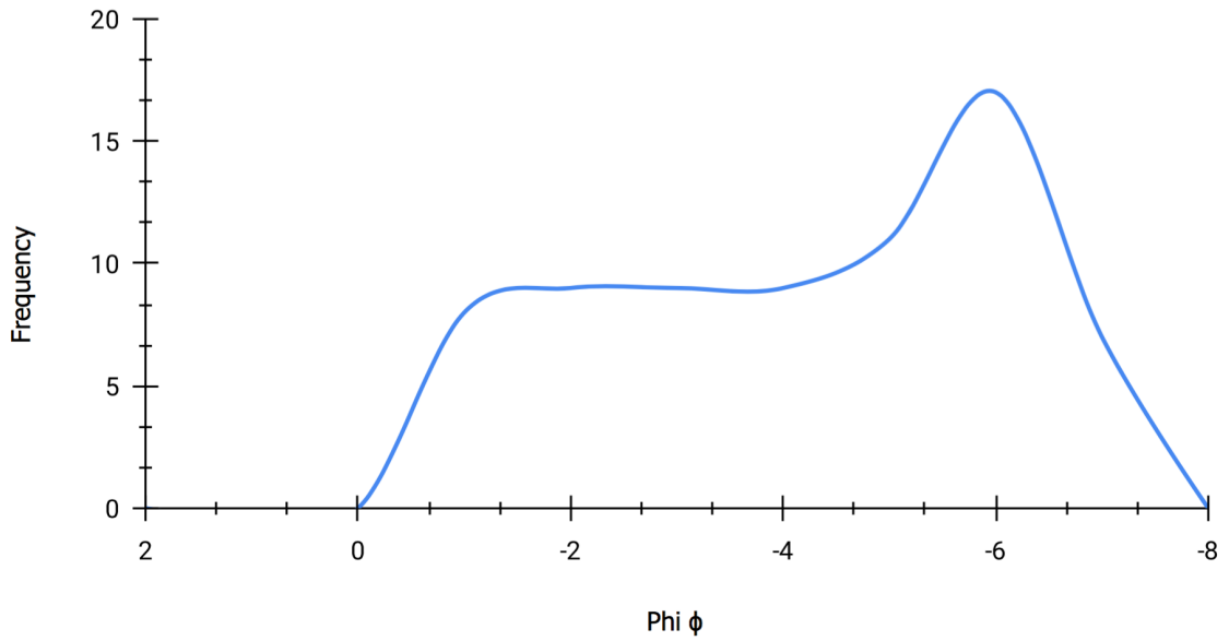
Appendix B. 37. West - Phi vs. Frequency individual graphs (CC15) Unit R.
