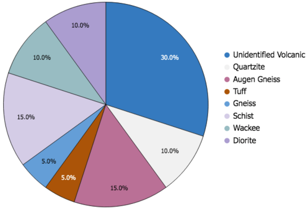
Appendix B. 53. West - Clast Composition individual pie charts with key (CC10) Unit R.
