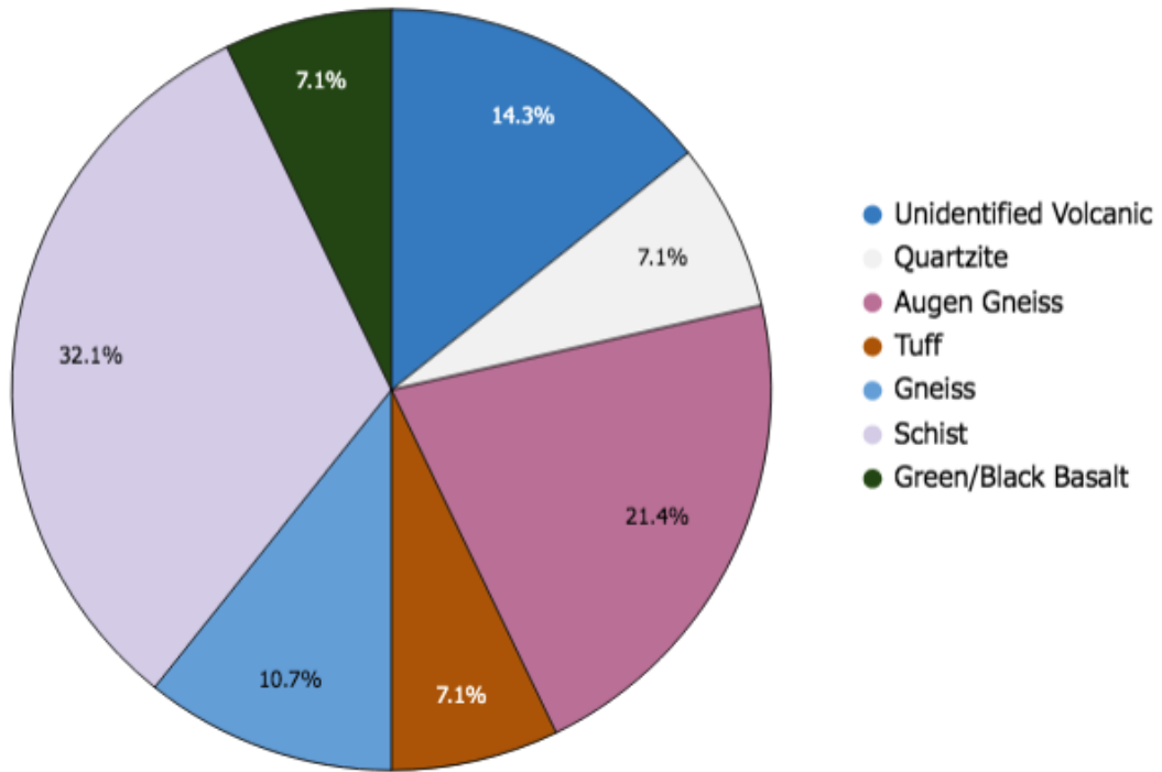
Appendix B. 59. East - Clast Composition individual pie charts with key (CC15) Unit R BRSS.
