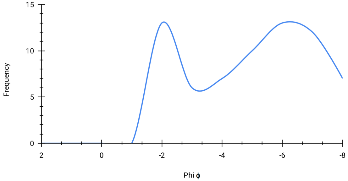
Appendix B. 44. West - Phi vs. Frequency individual graphs (CC21) Unit R.
