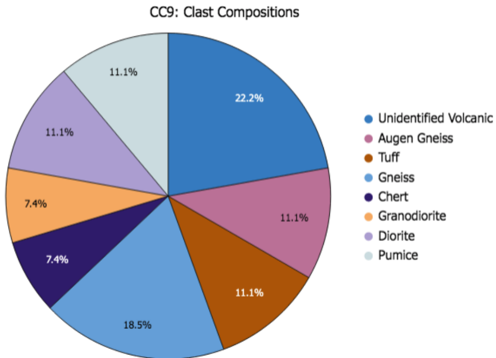
Appendix B. 52. West - Clast Composition individual pie charts with key (CC9) Unit L.
