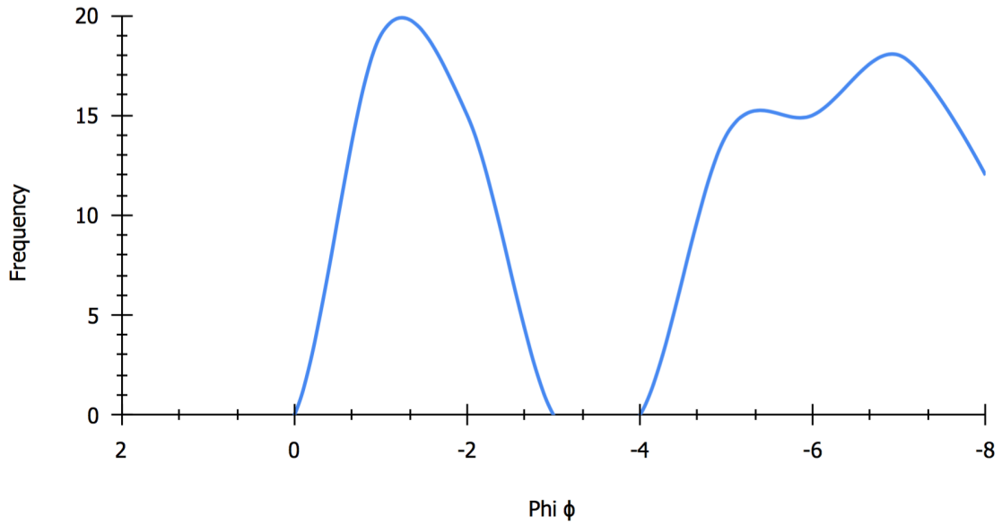
Appendix B. 27. West - Phi vs. Frequency individual graphs (CC6) Unit R.
