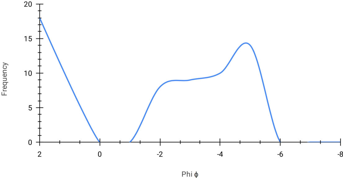
Appendix B. 32. West - Phi vs. Frequency individual graphs (CC22) Unit L.
