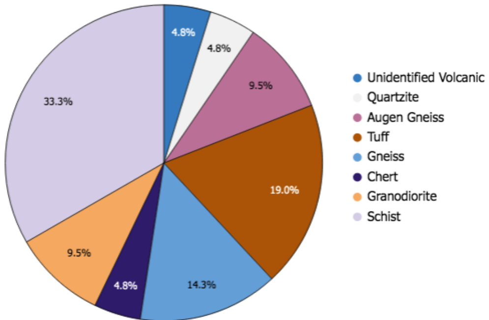
Appendix B. 54. West - Clast Composition individual pie charts with key (CC22) Unit L.
