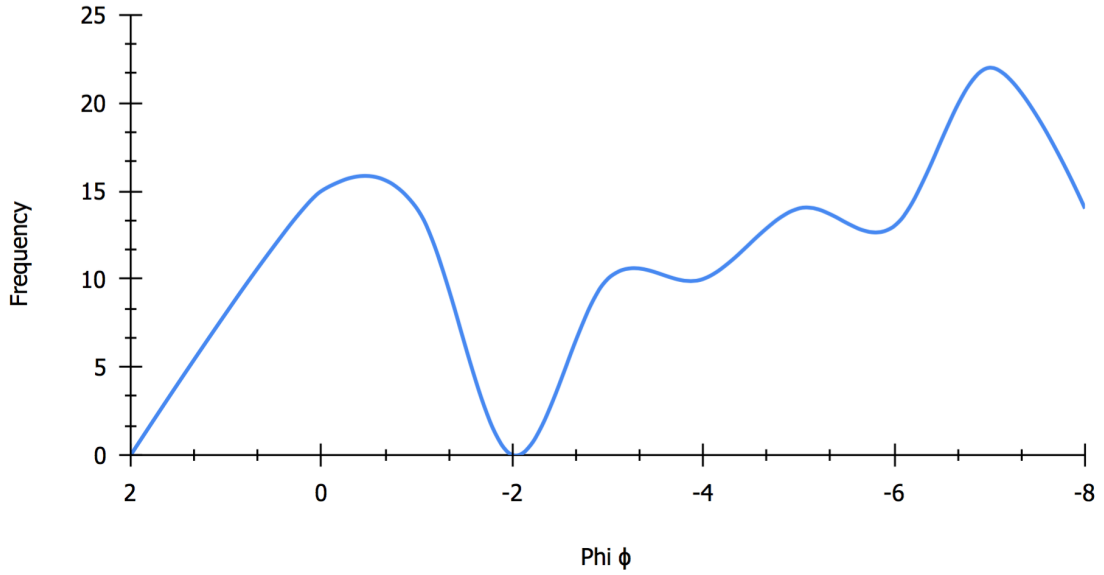
Appendix B. 33. West - Phi vs. Frequency individual graphs (CC11) Unit R.
