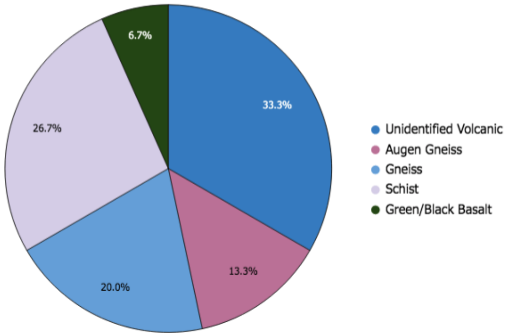
Appendix B. 62. East - Clast Composition individual pie charts with key (CC18) Unit L.
