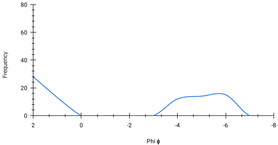
Appendix B. 24. West - Phi vs. Frequency individual graphs (CC3) Unit R.
