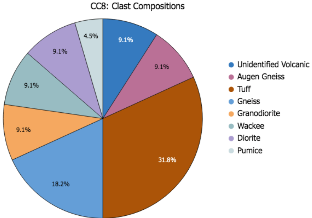
Appendix B. 51. West - Clast Composition individual pie charts with key (CC8) Unit R LRSS.
