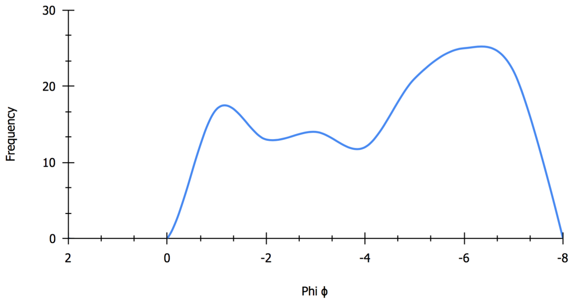
Appendix B. 34. West - Phi vs. Frequency individual graphs (CC12) Unit R.
