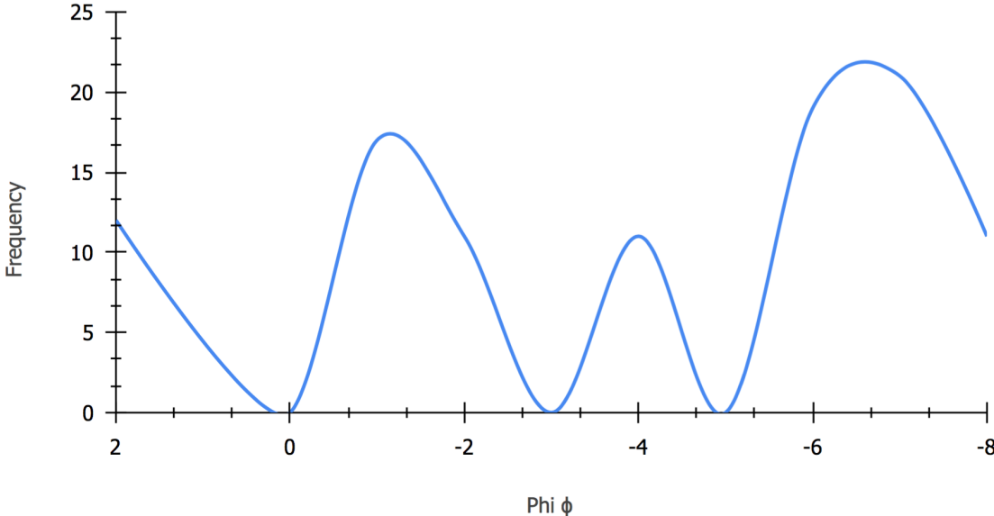
Appendix B. 29. West - Phi vs. Frequency individual graphs (CC8) Unit R.
