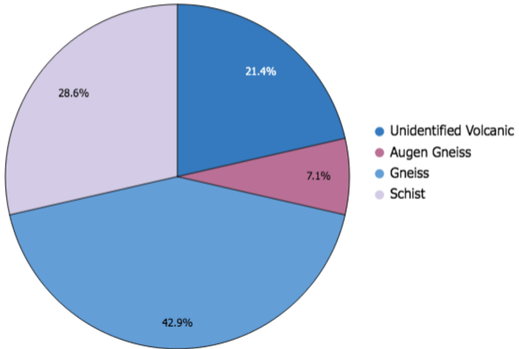
Appendix B. 61. East - Clast Composition individual pie charts with key (CC17) Unit R BRSS.
