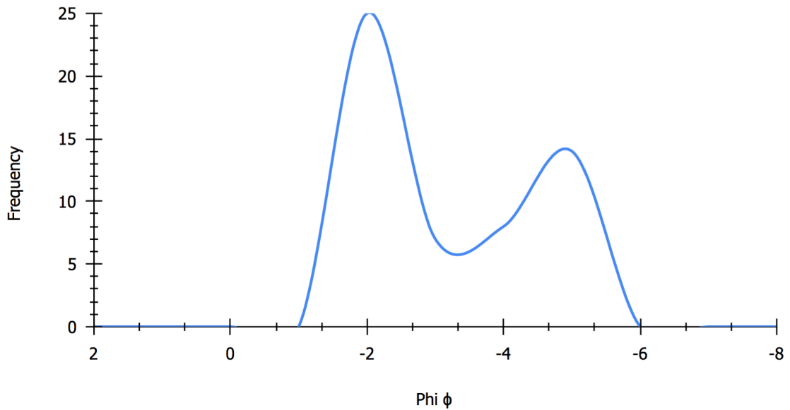
Appendix B. 39. West - Phi vs. Frequency individual graphs (CC17) Unit R.
