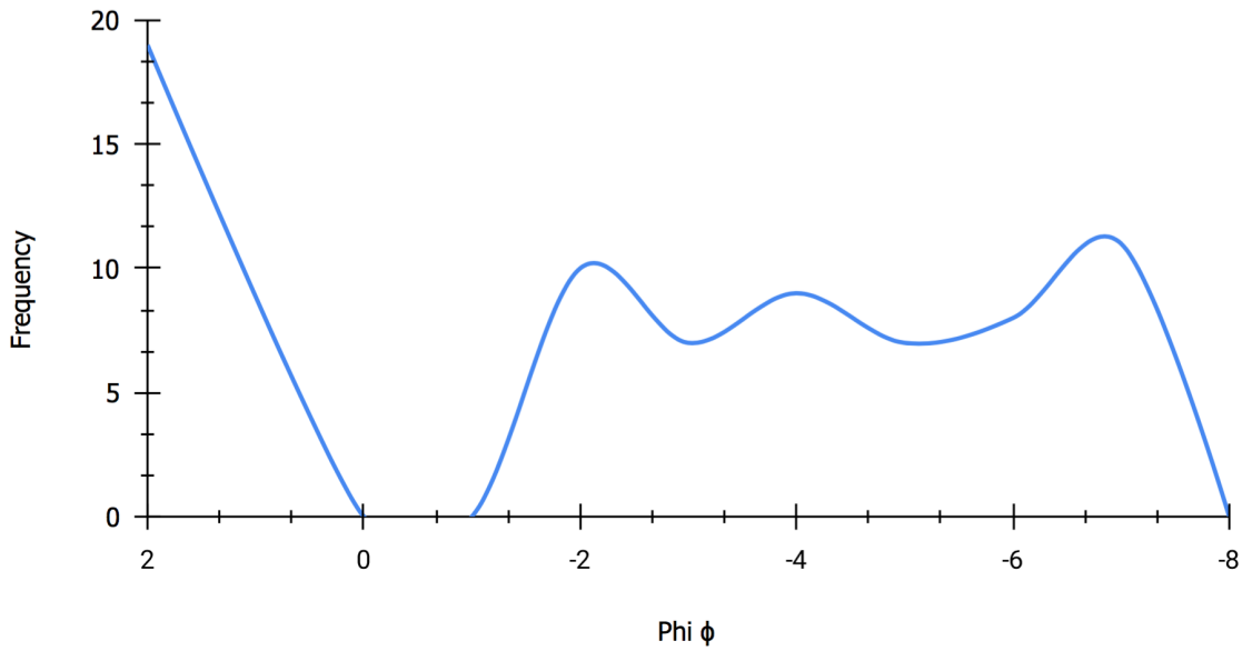
Appendix B. 41. West - Phi vs. Frequency individual graphs (CC19) Unit L.
