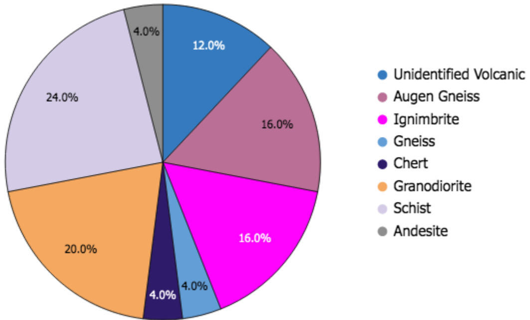
Appendix B. 55. East - Clast Composition individual pie charts with key (CC11) Unit R DRSS.
