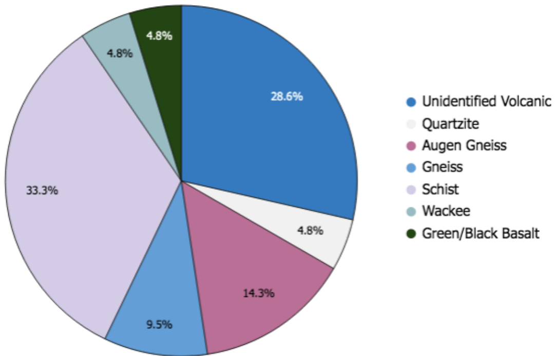
Appendix B. 60. East - Clast Composition individual pie charts with key (CC16) Unit R BRSS.
