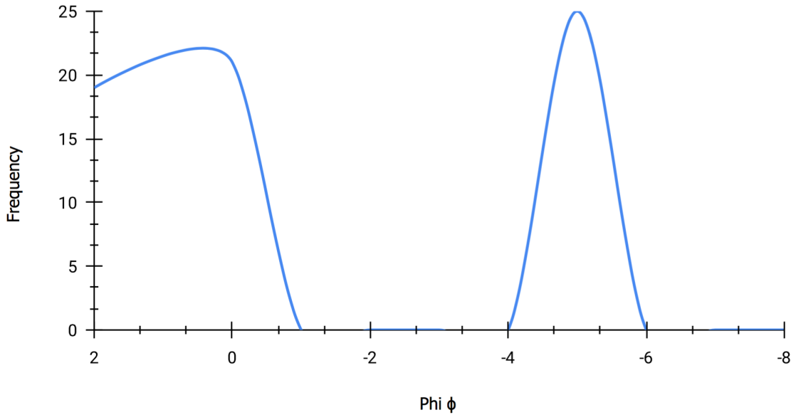
Appendix B. 40. West - Phi vs. Frequency individual graphs (CC18) Unit L.
